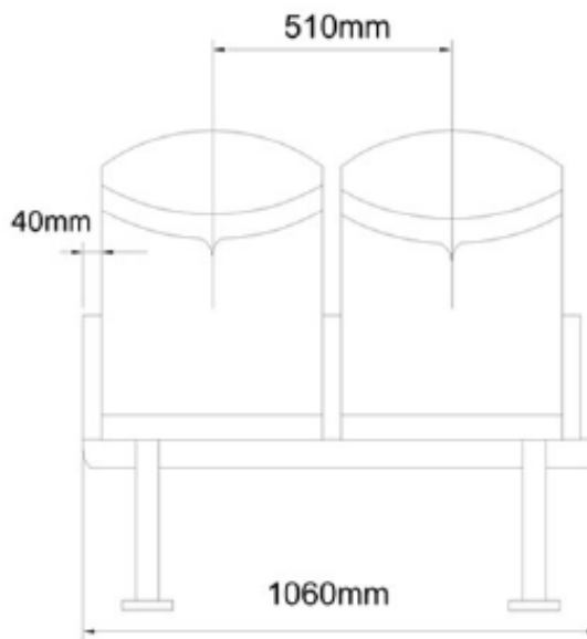
二客位联排 Two seats per row
