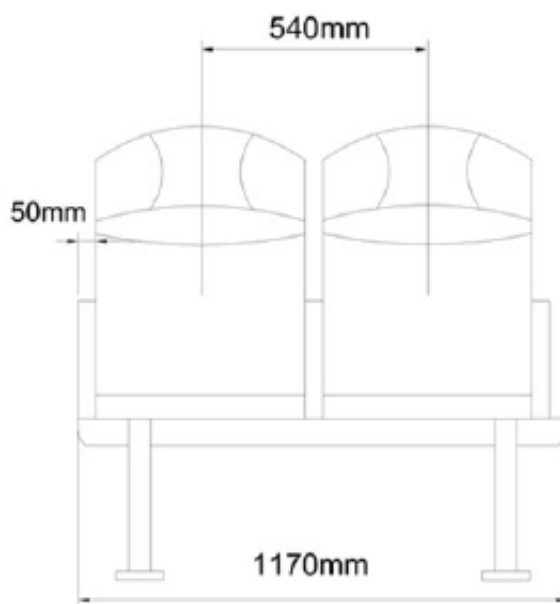
二客位联排 Two seats per row
